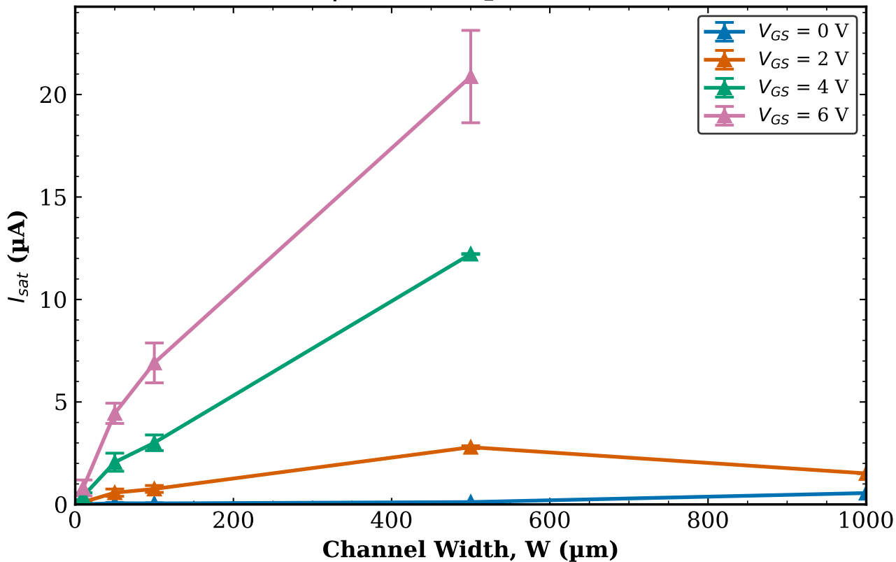
All Chips - Combined I_{sat} vs W | L = 160\text{ }\mu\text{m} (mean \pm std)
